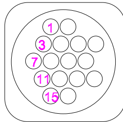
AMP 206036-1 connector pin layout on base of PTE-300 pan tilt head
